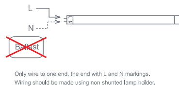
Diagram 3 – Single tube wiring
